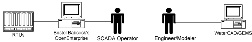
Fig 1: Schematics of Data transfer without a hard wire connection between the computer having modeling software and the computer having SCADA data
