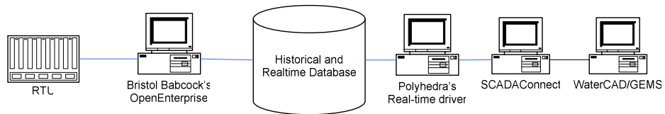
Fig 3: Schematics of automated implementation in SCADAConnect
